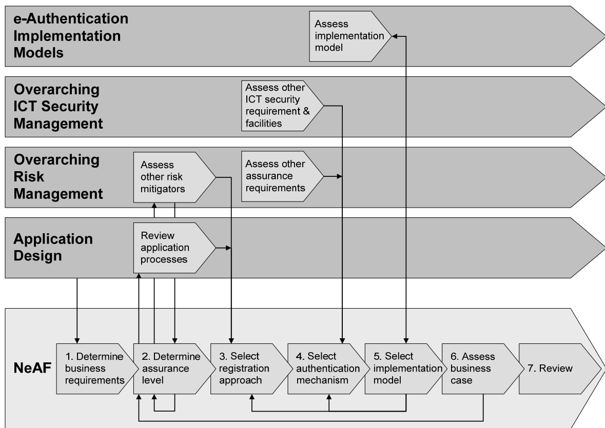
Figure 1: NeAF process
