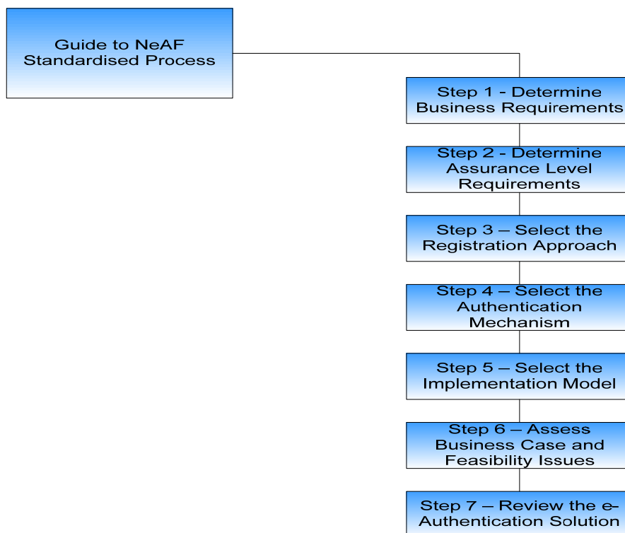
Figure 2: Methodology
